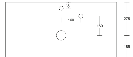
CUT OUT SPECIFICATIONS
