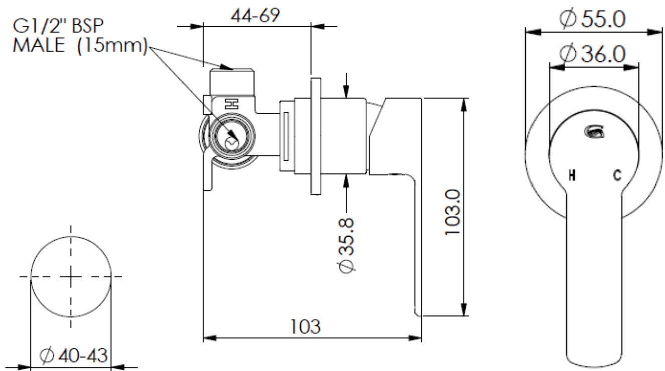
Mounting Hole
