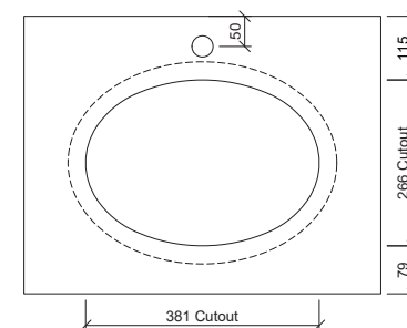
Cut Out Specifications
