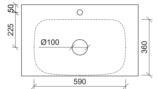
Taphole Behind
