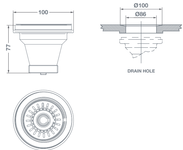
38mm Basket Strainers
