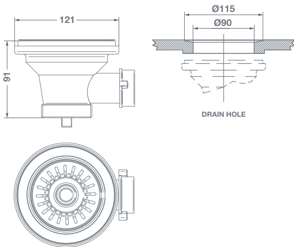
90mm Basket Strainers
