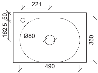
Taphole Offset
