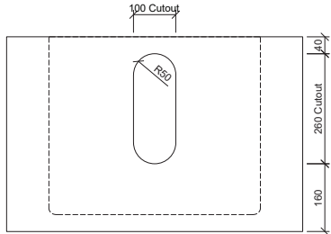
Cut Out Specifications
