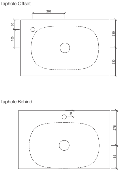
Cut Out Specifications
