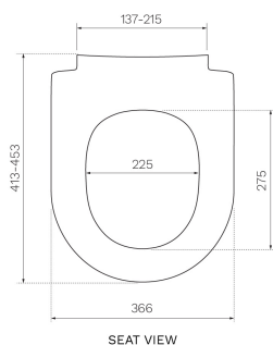
SEAT VIEW
