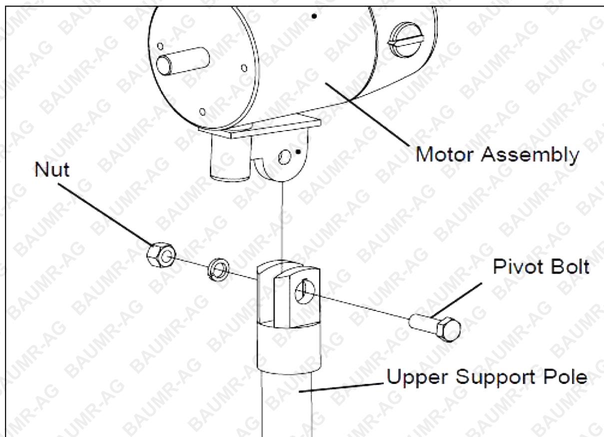
Attaching Motor to Motor Support Assembly
