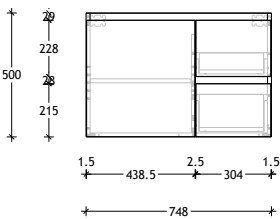
750 Centre HLYE750WH
