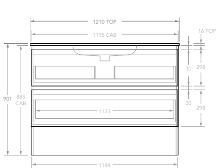
1200 Centre HLY1200WKS
