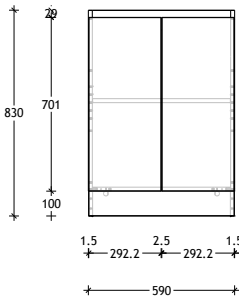
600 Centre HLYE600WK
