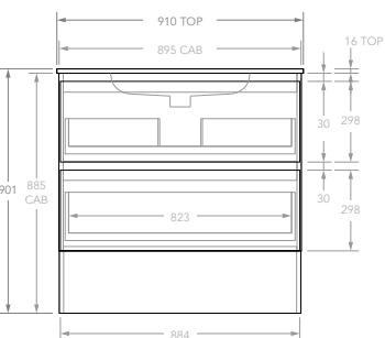
900 Centre HLY0900WK
