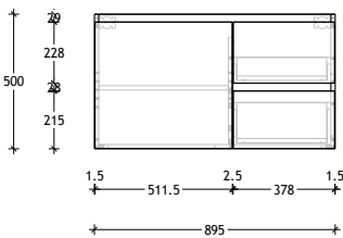
900 Centre HLYE900WH
