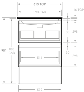
600 Centre HLY0600WK
