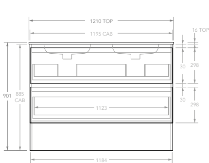
1200 Double HLY1200WKD
