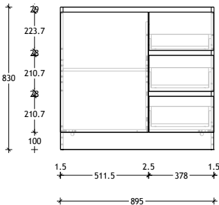
900 Centre HLYE900WK
