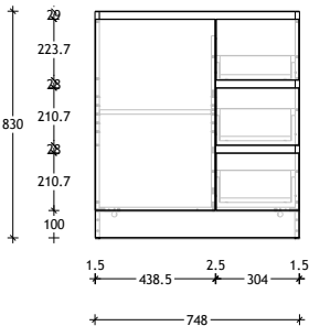
750 Centre HLYE750WK
