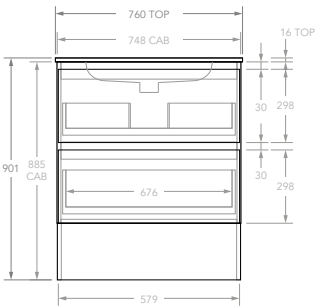
750 Centre HLY0750WK
