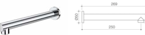
Luna Lever Bath Outlet 250mm ● 90337C
