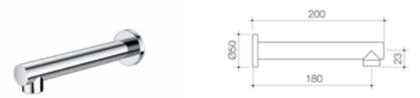
Luna Lever Basin Outlet 185mm WELS 5 star rated, 4.5-6L/min ● 90335C5A
