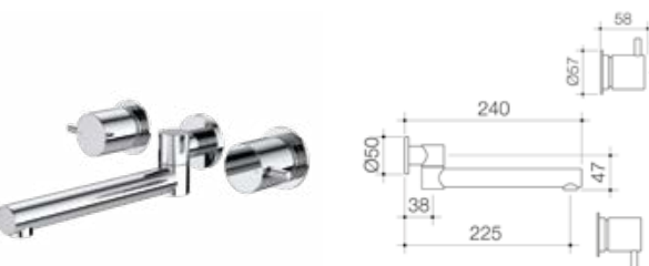
Luna Lever Laundry Tap Set WELS 4 star rated, 6-7.5L/min ● 90331C4A ● 90331BL4A
