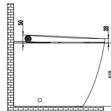
Neion SQ wall faced intelligent toilet with remote and Arcisan concealed cistern
