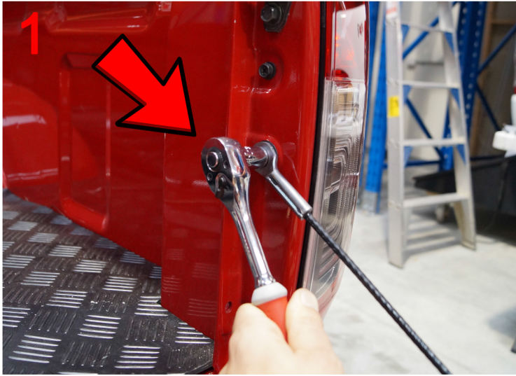
1: Remove cable bolt from the tub
