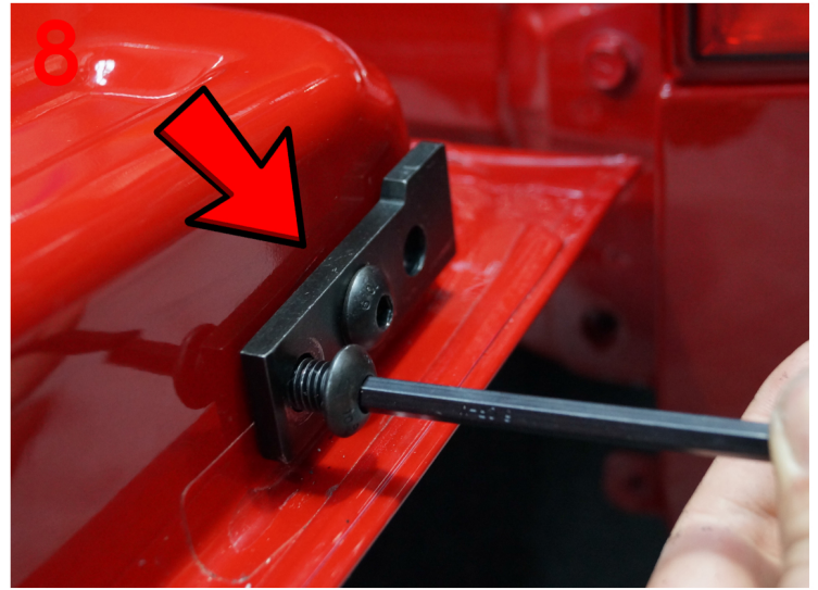
8: Insert only 2 bolts through the bracket as shown. The 3rd bolt is installed later in step 12
