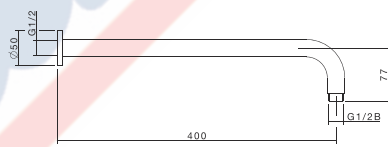
Titan Wall Shower Arm - Right Angle 99021SS
