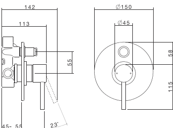
Titan Bath/Shower Mixer with Diverter 99002SS
