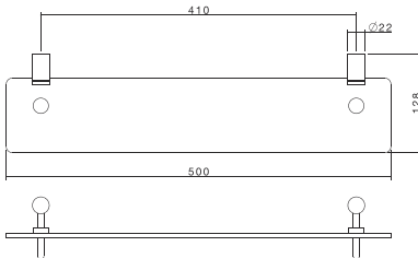
Titan Glass Shelf 99016SS
