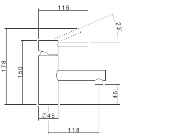
Titan Basin Mixer WELS 6 star rated, 4.5L/min 99000SS6A
