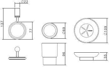
Titan Soap Holder/ Tumbler Pack 99014SS
