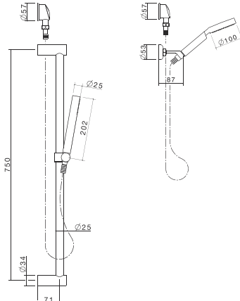
Titan Rail Shower with Microphone Hand Piece WELS 3 star rated, 9L/min 99022SS3A
