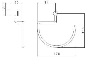
Titan Hand Towel Ring 99015SS
