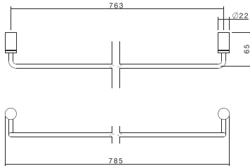
Titan Single Towel Rail 99011SS
