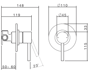
Titan Bath/Shower Mixer 99001SS
