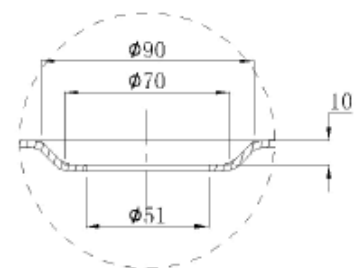
Enlarged Drawing A
