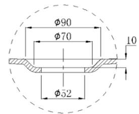
Enlarged Drawing A
